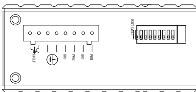
Terminal Block
