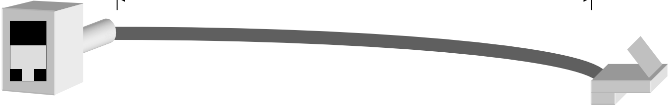
CAT5 UTP 6" Cable terminated in a Modular RJ-45 Plug and RJ-45 Jack with translation wiring for Cisco/Sun Devices Part # 449016
